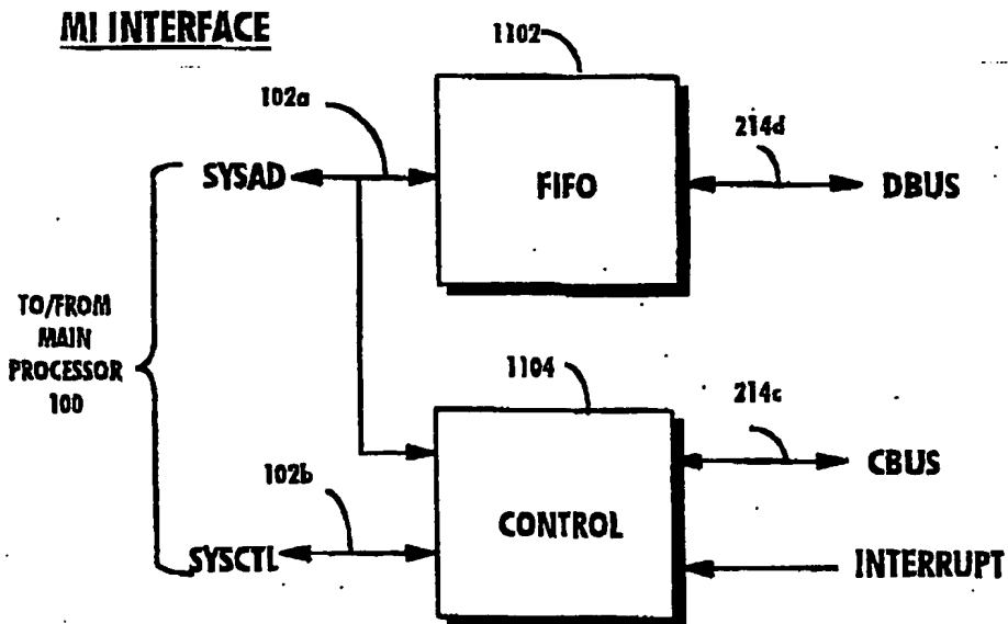
Fig. 38 EXAMPLE CPU INTERFACE
